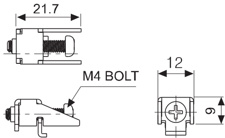
Fixing bracket
